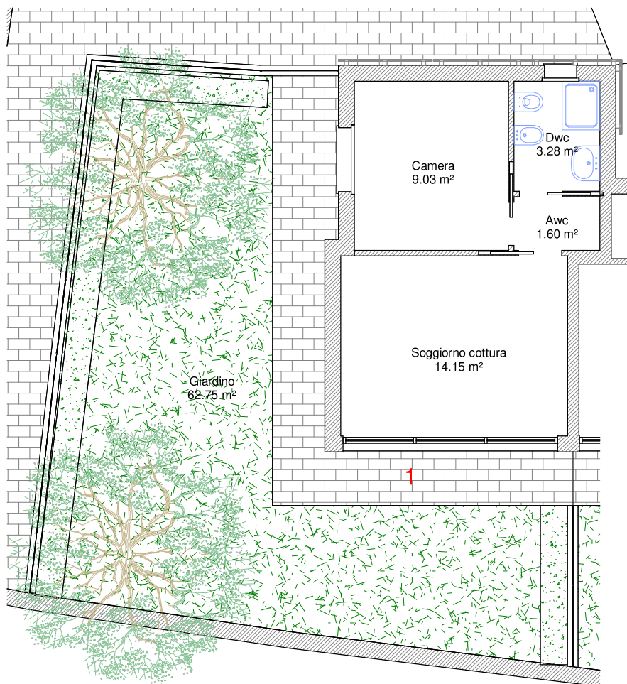
PIANO TERRENO
